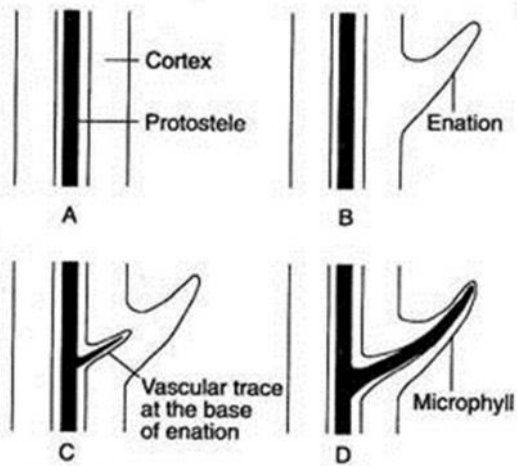
Enation theory : A–C. Stages in the origin of microphyll. A. Axis of Rhyniopsida , B. Axis of Zosterophyllopsida , C. Axis of Asteroxylon , D. Axis of Lycopsidea showing a microphyll
